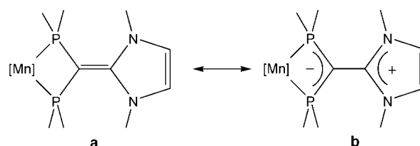
Figure 4. Resonance structures of imidazoline-functionalized diphosphane complexes. [Mn] = [Mn(CO) 4 ] + .
