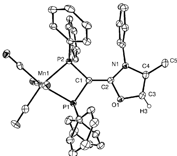
Figure 3. A view of the structure of the cation of 2b . Selected bond lengths [Å] and angles [°]: P1–C1 1.781(4), P2–C1 1.770(4), C1–C2 1.385(6), N1–C2 1.338(6), N1–C4 1.422(5), O1–C2 1.364(5), O1–C3 1.398(6), C3–C4 1.335(7); P1–Mn–P2 71.09(4), P1–C1–P2 99.7(2), N1–C2–O1 107.9(3), N1–C2–C1 135.4(4), O1–C2–C1 116.7(4).
