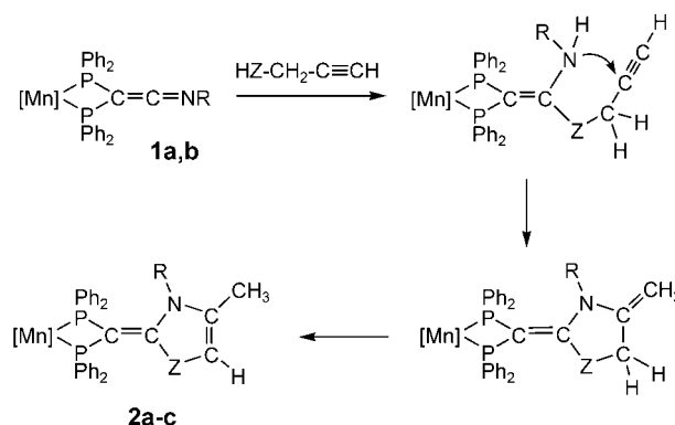
Scheme 1. Proposed mechanism for the formation of complexes 2a–c . [\text{Mn}] = [\text{Mn}(\text{CO})_4]^+ . 1a : R = Ph; 1b : R = p -tolyl. 2a : R = Ph, Z = NH; 2b : R = Ph, Z = O; 2c : R = p -tolyl, Z = NMe.
