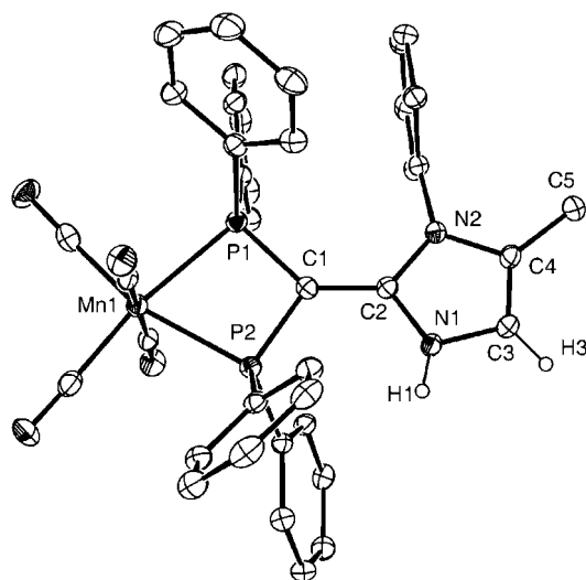
Figure 2. A view of the structure of the cation of 2a . Selected bond lengths [Å] and angles [°]: P1–C1 1.749(3), P2–C1 1.761(3), C1–C2 1.429(4), N1–C2 1.342(3), N1–C3 1.382(4), N2–C2 1.371(3), N2–C4 1.416(3), C3–C4 1.333(4); P1–Mn–P2 69.84(2), P1–C1–P2 99.23(13), N1–C2–N2 105.4(2), N1–C2–C1 125.0(2), N2–C2–C1 129.5(2).
