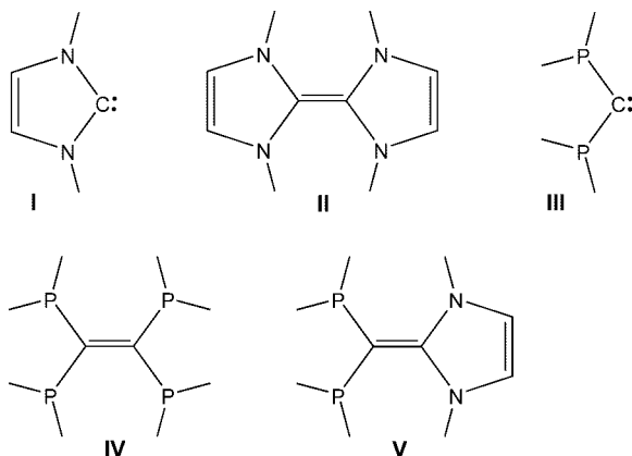
Figure 1. Schematic representation of imidazol-2-ylidenes and diphosphinylcarbenes, and their coupling products.
