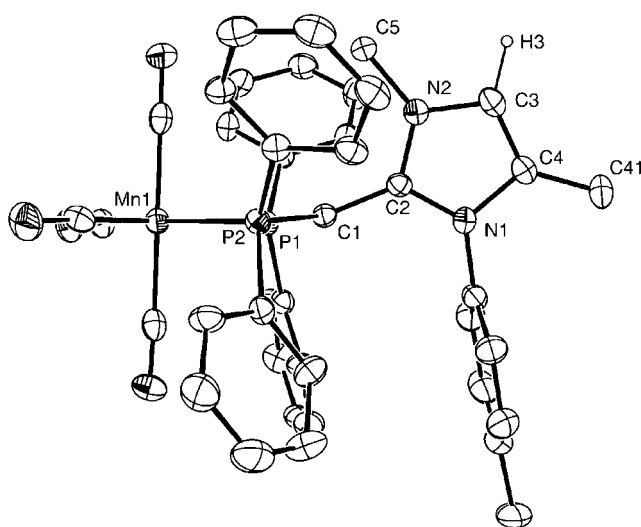
Figure 5. A view of the structure of the cation of 2c . Selected bond lengths [Å] and angles [°]: P1–C1 1.755(7), P2–C1 1.744(7), C1–C2 1.461(9), N1–C2 1.351(8), N1–C4 1.404(9), N2–C2 1.346(8), N2–C3 1.385(9), C3–C4 1.356(9); P1–Mn–P2 69.90(7), P1–C1–P2 99.9(1), N1–C2–N2 105.9(6), N2–C2–C1 124.9(6), N1–C2–C1 129.2(6).
